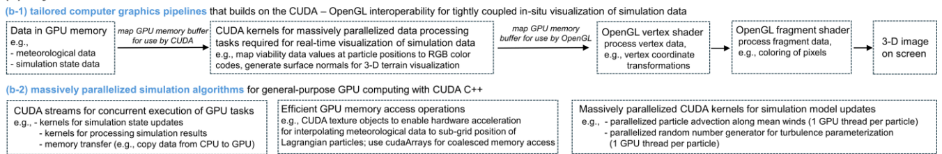
Figure 2: Conceptual summary of AgPaDS heterogeneous CPU-GPU implementation.
