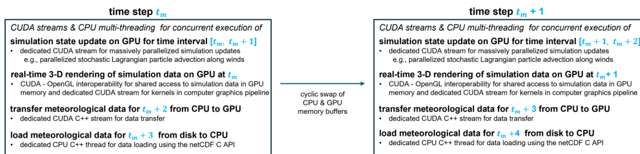
405 Figure 3: Time-streaming with cyclic swap of CPU & GPU memory buffers for concurrent loading of data from disk to CPU, transfer of from CPU to GPU, simulation state update and real-time rendering on GPU.
