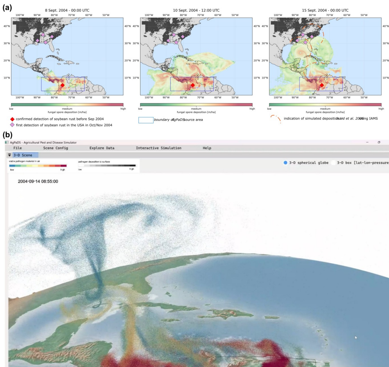
745 Figure 7: AgPaDS simulation of atmospheric transport of Phakopsora pathogenic fungal spores caused by hurricane Ivan in 750 in 2004 that has likely transmitted soybean rust into the USA. (a) cumulative pathogen deposition at different time-steps in comparison with published confirmed soybean rust detection sites and sketch of IAMS simulation results (Isard et al., 2005); (b) snapshot of AgPaDS GUI with 3-D in situ visualization of simulated atmospheric pathogen transport. See Movie 15 ( https://av.tib.eu/media/72272 ) for a screenshot recording of the AgPaDS GUI for this simulation, demonstrating the dynamic in situ 3-D visualization
